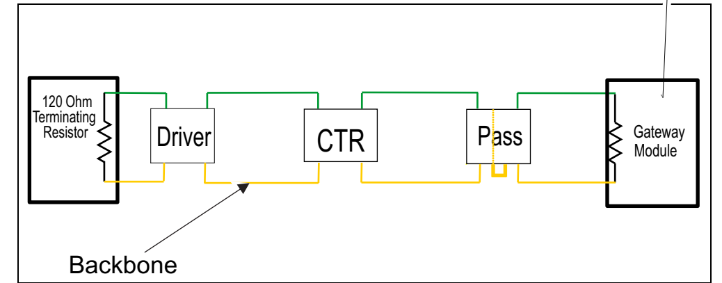
J1939-250K Multiplexing System connections
