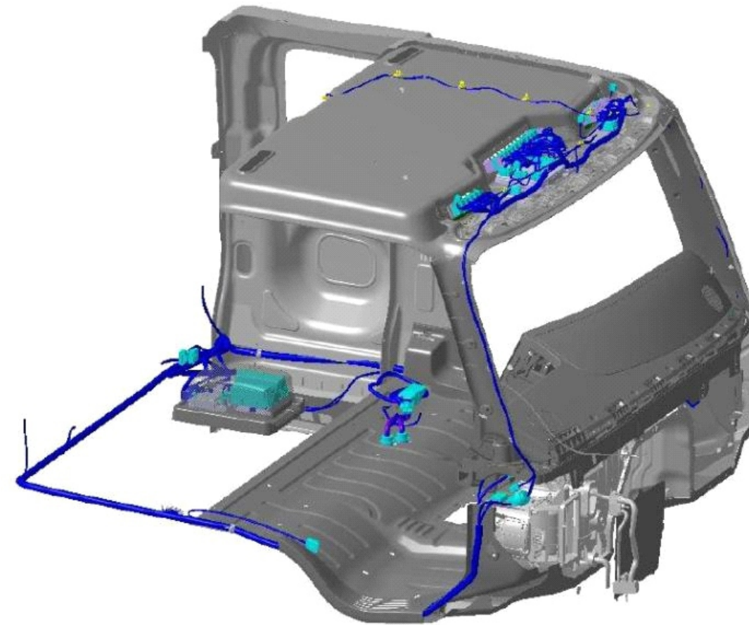
Extended Cab wired with SmartPlex
