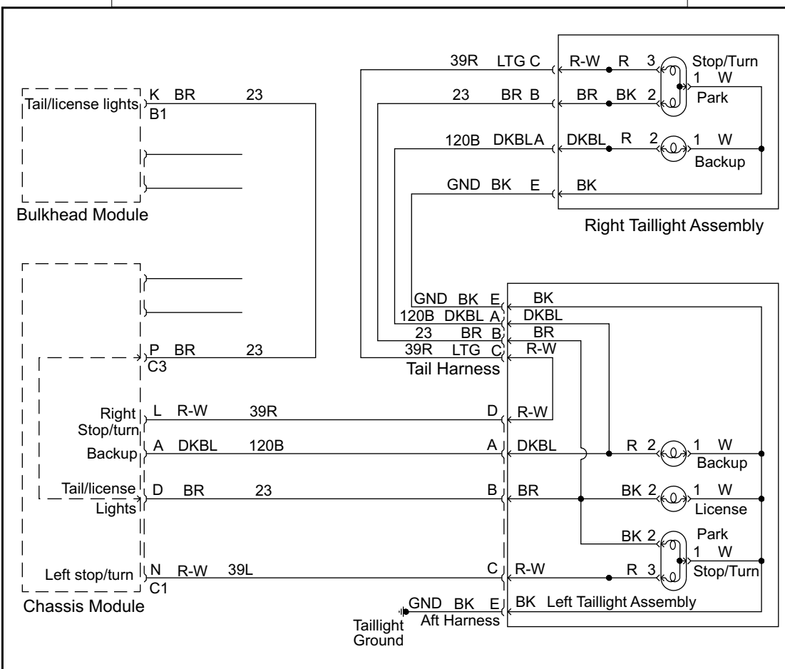
Lighting Outputs For Integrated RearLights (Combination stop/turn signal)
