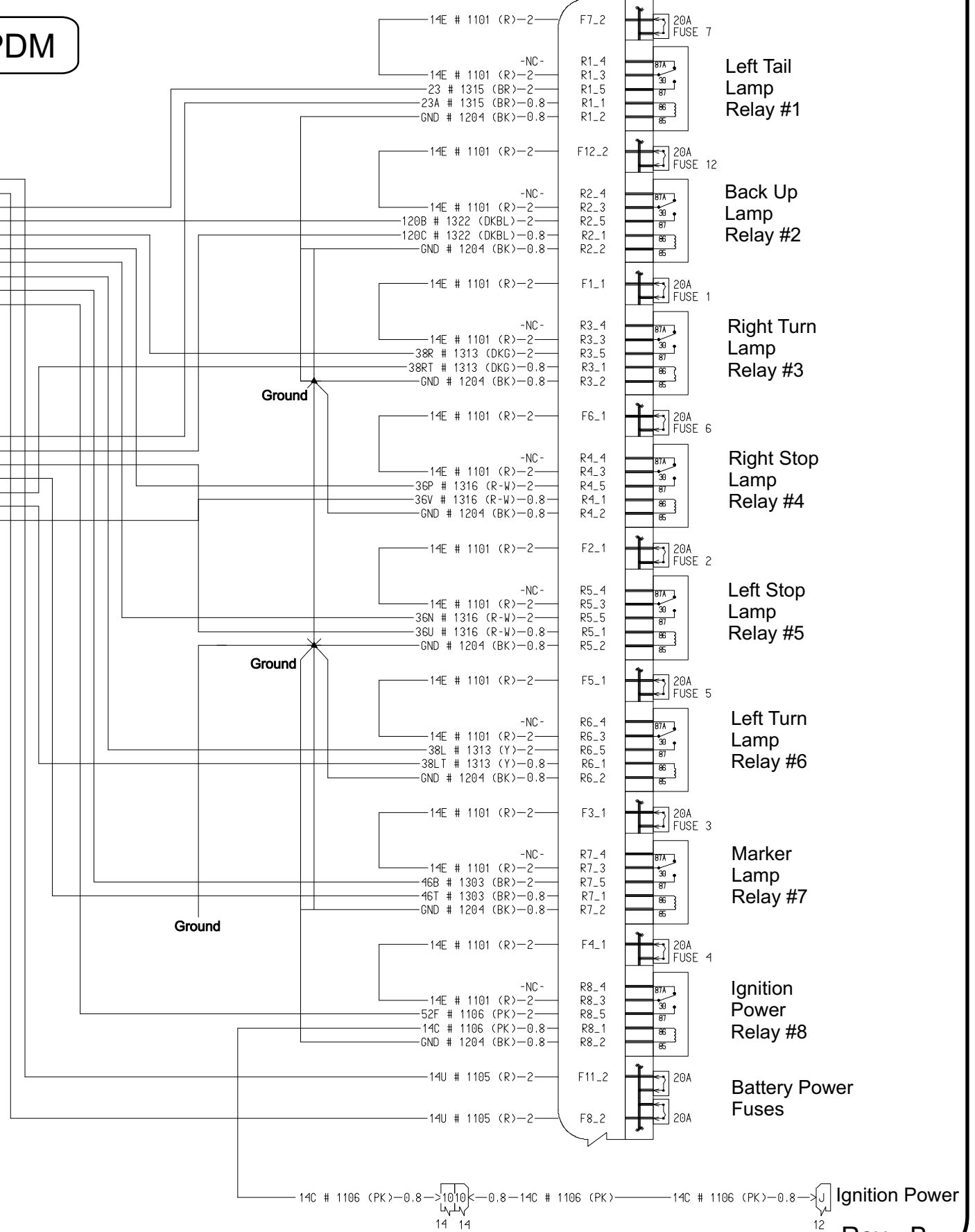
353-026 and 353-027 Schematic
