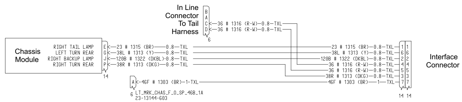
353-022 and 353-023 Schematic
