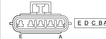
Rear Light Connector (combination stop/turn signal)
