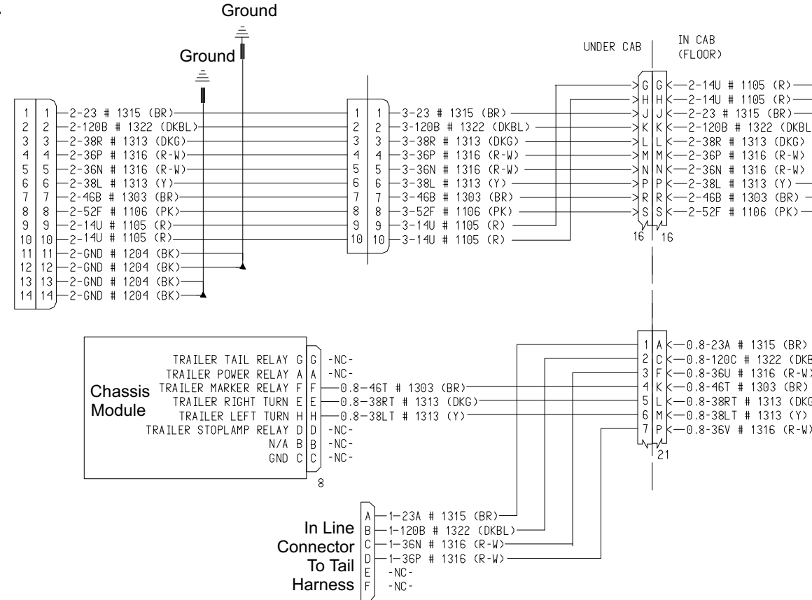
353-026 and 353-027 Schematic
