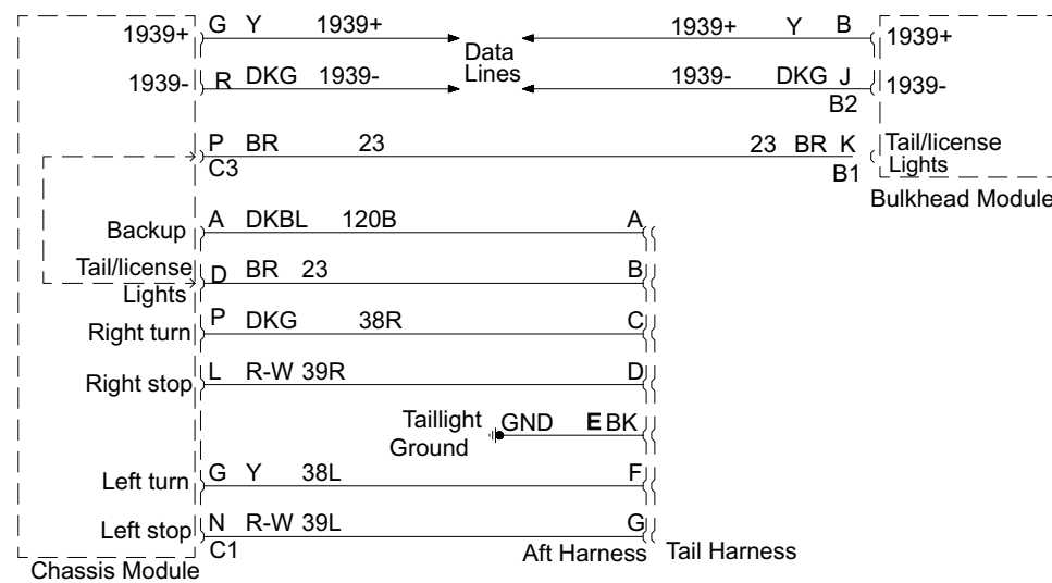
RearLighting Connection (separate stop/turn signal)
