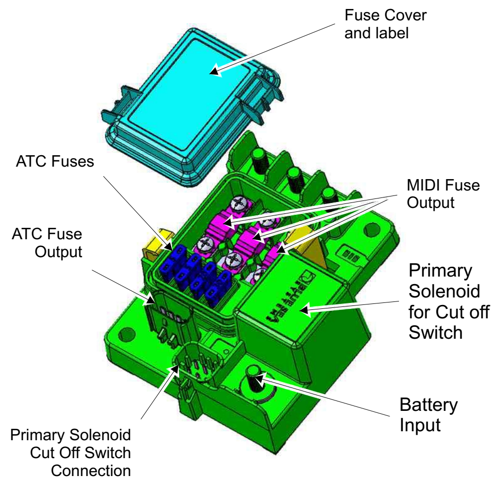
INSTALLATION WITHOUT DISCONNECT SWITCH
