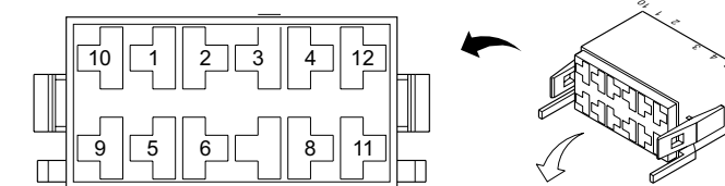
Smart Switch Pinout for a Two Position Switch Pins
