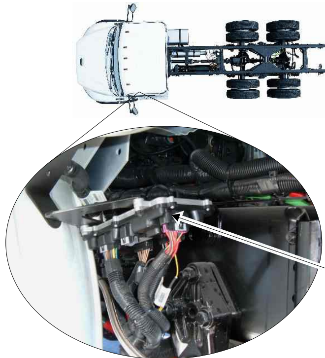
The CHM is under the cab to improve durability and free up frame space
