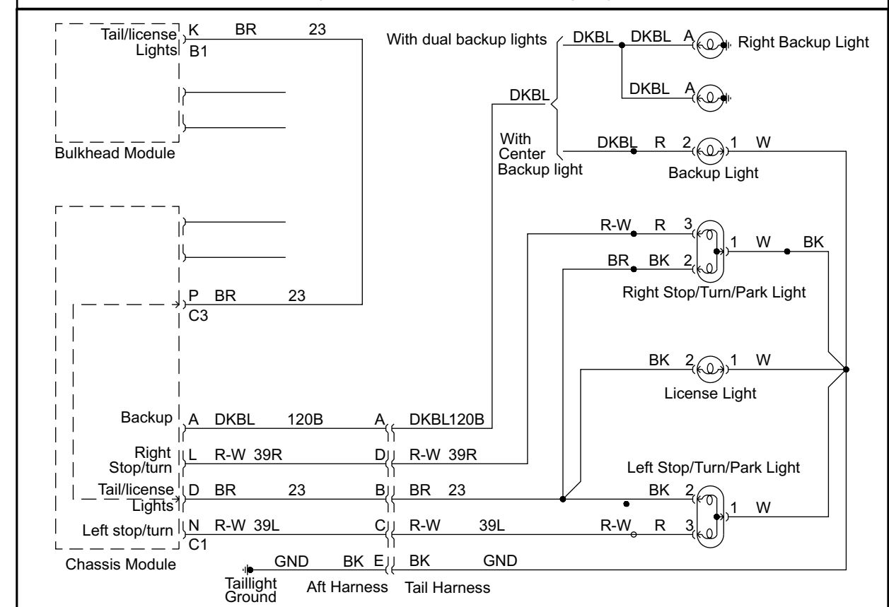
Lighting Outputs For Individual RearLights (Combination stop/turn signal)
